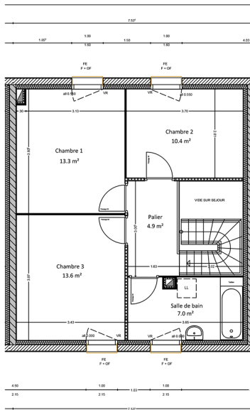
PLAN R+1
